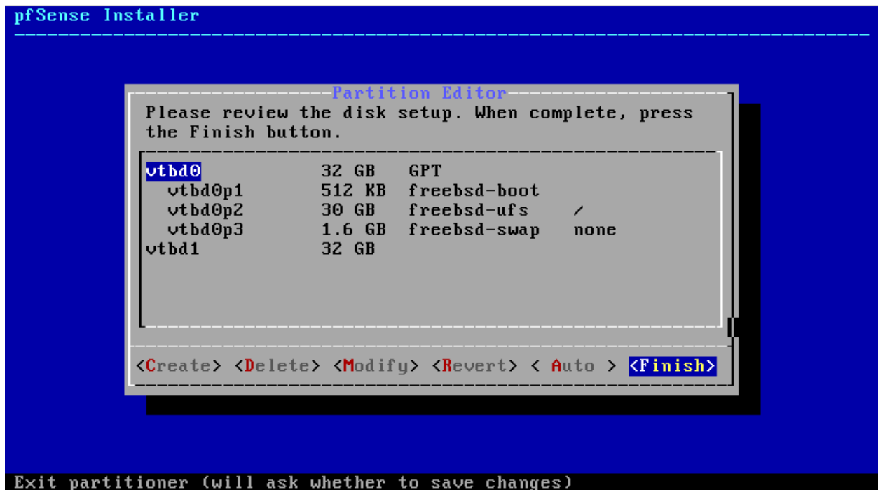
Fig. 12: Partition Editor
