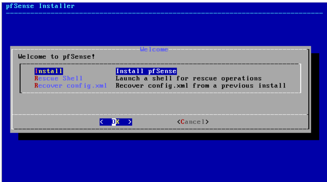
Fig. 2: Rescue Options
