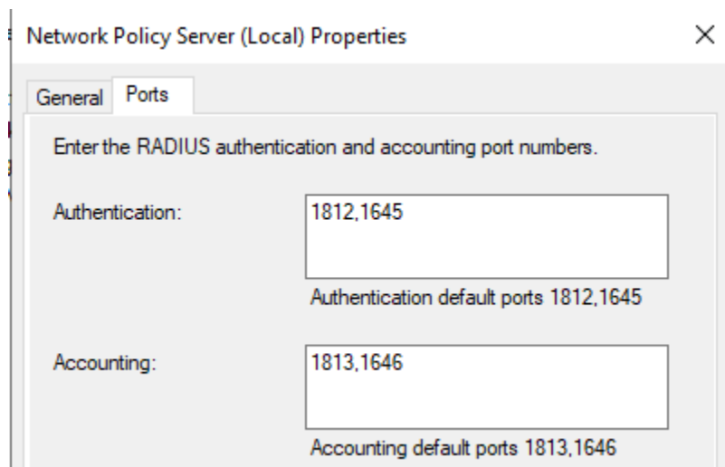
Fig. 93: NPS Ports
