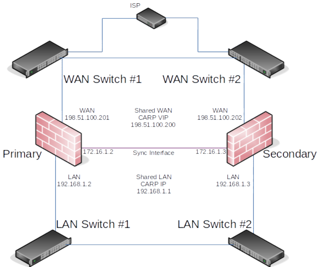
Fig. 3: Diagram of HA with Redundant Switches
