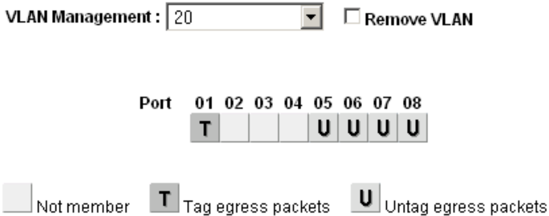
Fig. 109: Configure VLAN 20 Membership
