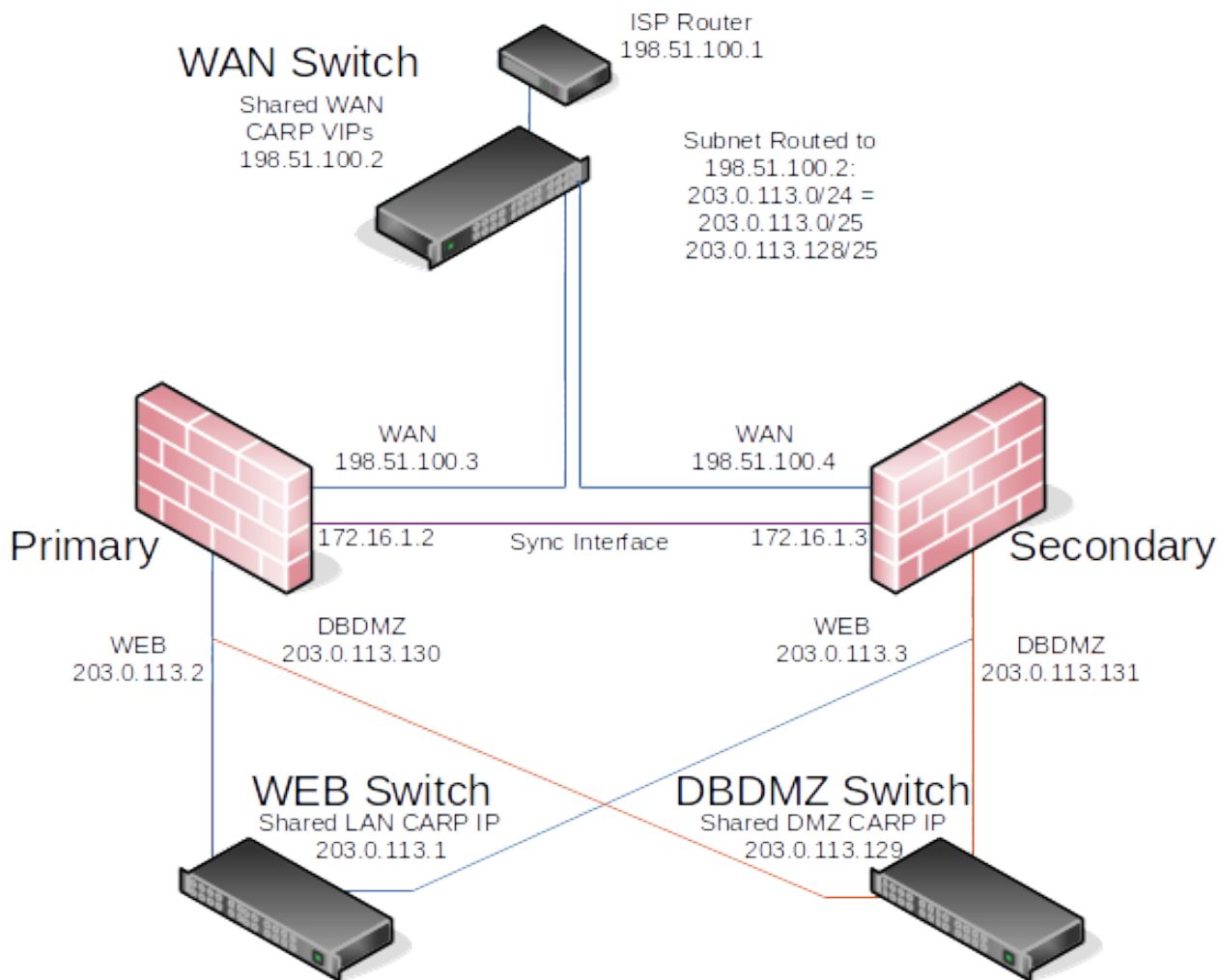
Fig. 11: Diagram of HA with Routed IPs
