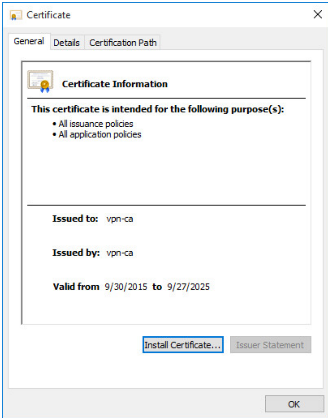
Fig. 13: Certificate Properties
