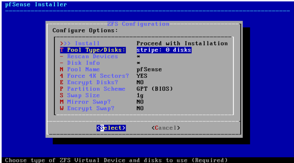
Fig. 5: ZFS Configuration
