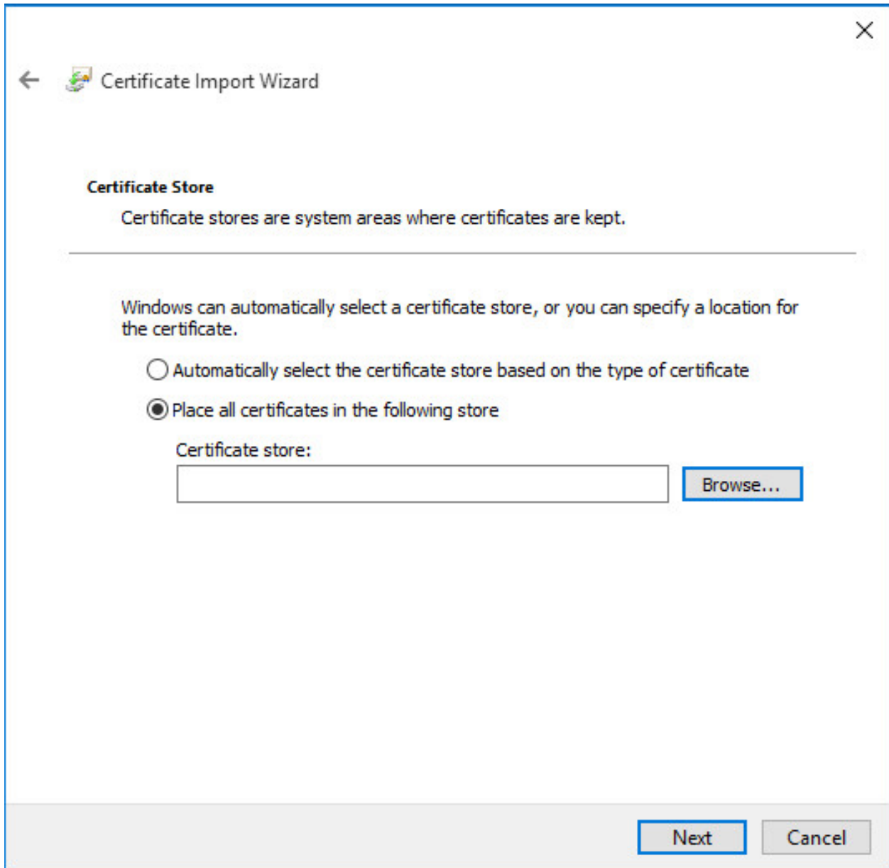
Fig. 15: Certificate Import Wizard - Browse for the Store
