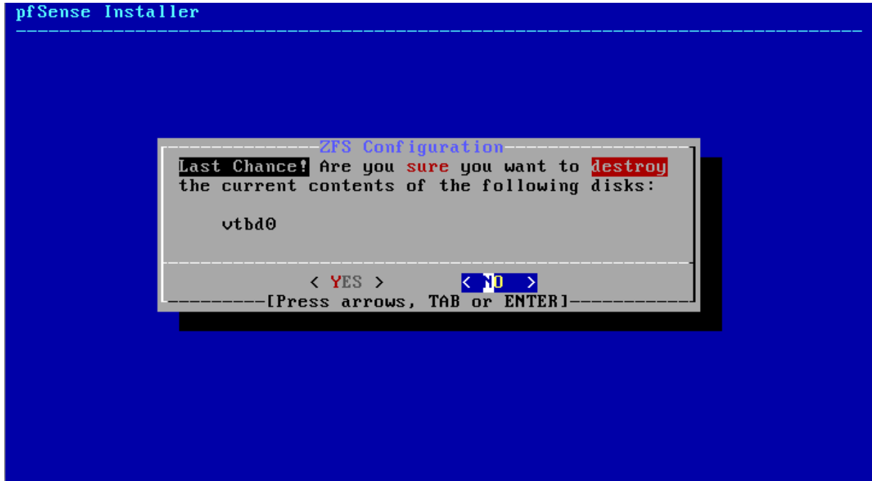
Fig. 8: ZFS Confirmation
