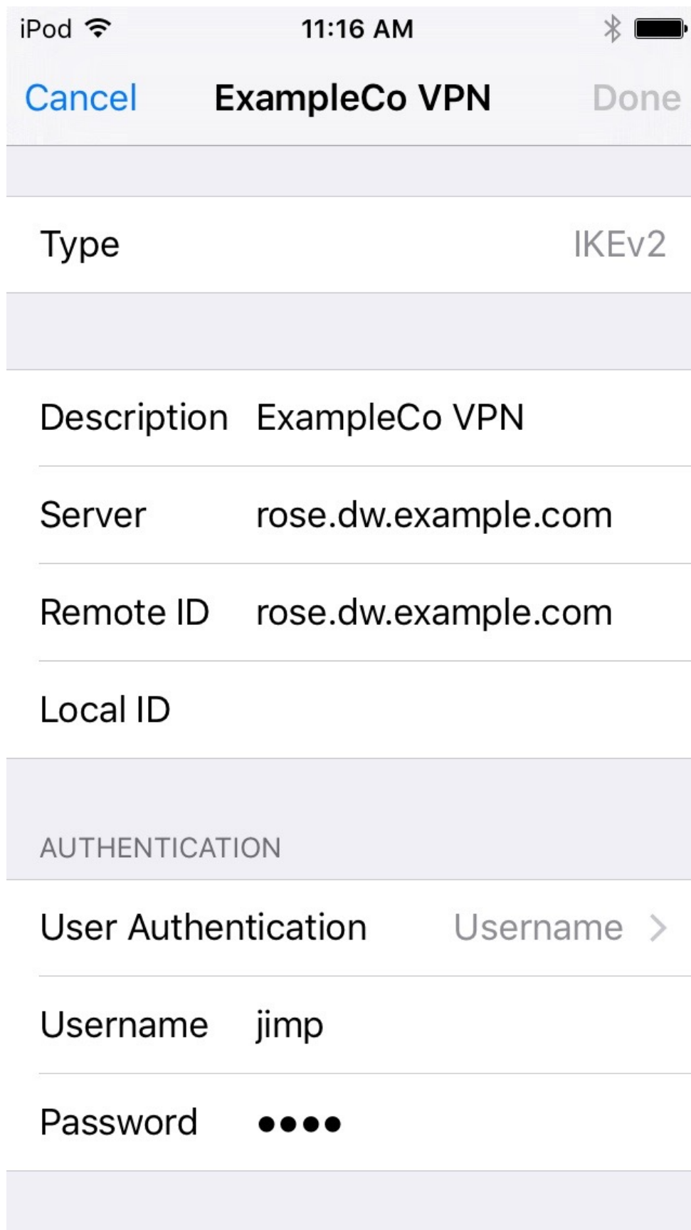
Fig. 34: iOS IKEv2 Client Settings
